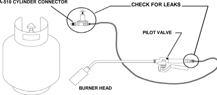
CGA-510 CYLINDER CONNECTOR
